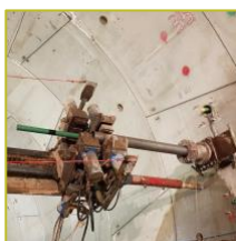
Waterproofing injections
